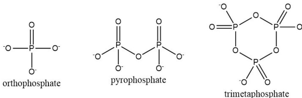
Figure 2. Structural formulas of the unprotonated forms of phosphate, a phosphate dimer, and a cyclic phosphate trimer.
