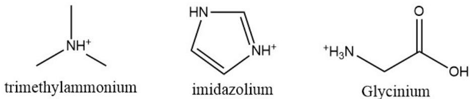
Figure 1. Structural formulas of several protonated amines.
